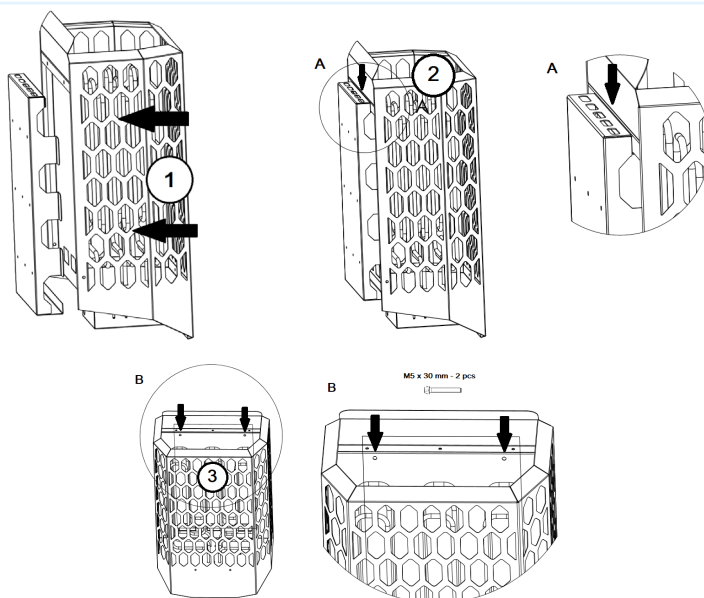
Fig. 3 Mounting the heater in a wall bracket.
