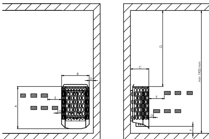
Fig. 1 Safe positioning of the heater in the room.
