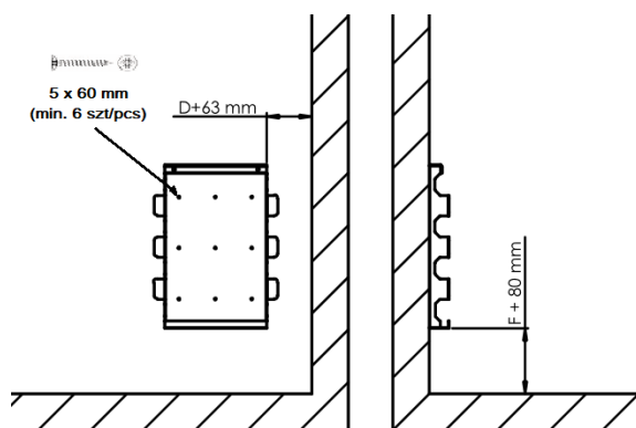
Fig. 2 Location of the holes for the heater wall bracket.
